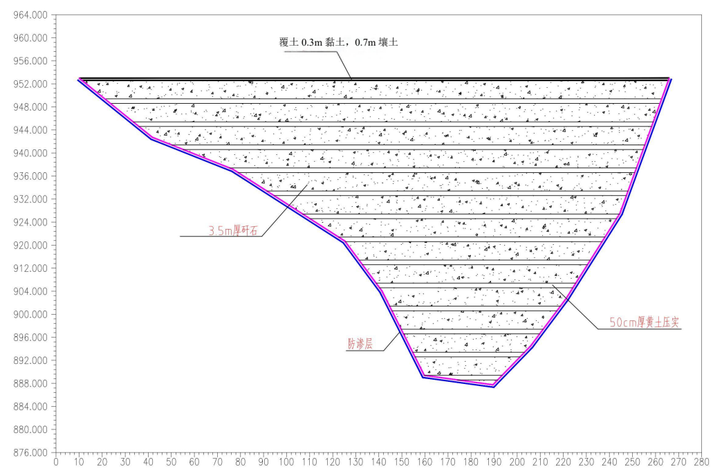
场区矸石堆放典型横断面图
